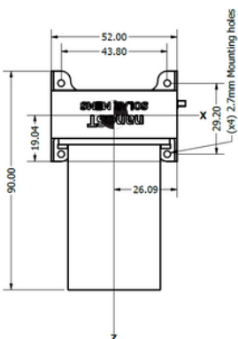
nanoST with cubesat baffle
