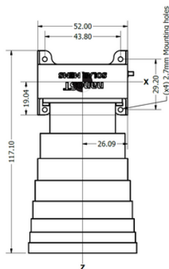
nanoST with non-cubesat baffle
